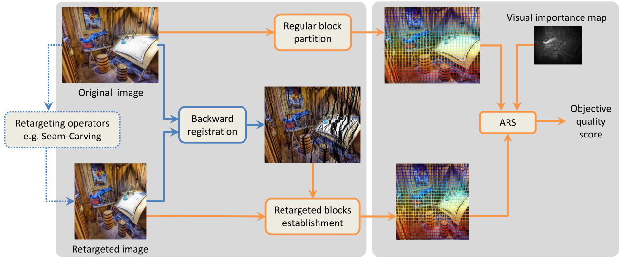
Fig. 1. The framework of the proposed method. The backward registration (blue solid path) aims to reveal the geometric change during the image retargeting and under the guidance of the estimated geometric change, ARS metric (orange solid path) obtains the objective quality score.
