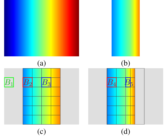
Fig. 8. A toy example for ARS metric. (a) Original image ( 512 \times 384 ). (b) Retargeted image ( 192 \times 384 ). We crop out the middle half of the original image as (c) and then the scale the right half by 50% width reduction as (d). The original image is divided into 64 \times 64 regular non-overlapped blocks as (c) and the corresponding retargeted blocks are shown in (d). The block B_1 is totally removed, B_2 is well-preserved as B_4 , and B_3 is scaled to B_5 .
