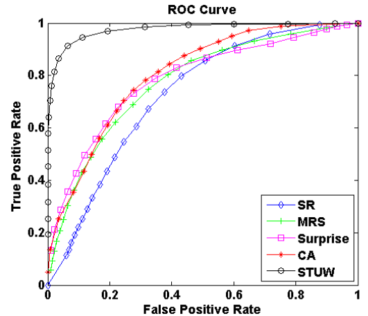
Fig. 9. ROC comparison of spatiotemporal saliency models.
