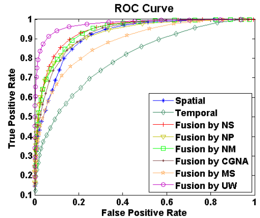
Fig. 6. ROC comparison of spatial saliency, temporal saliency, and spatiotemporal saliency by different fusion methods.
