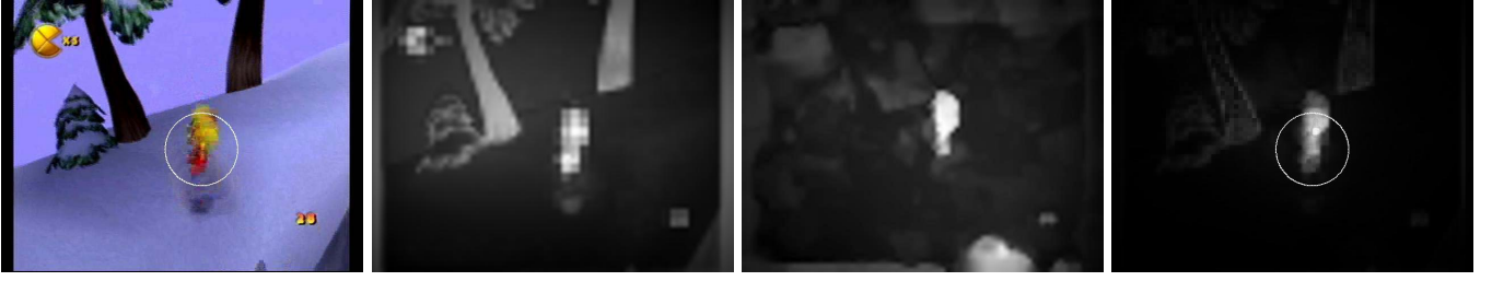
Fig. 4. Sample saliency maps. Column 1: original video frame with human fixation point marked with a circle; Column 2 - 4: spatial, temporal, and overall saliency maps, respectively.
